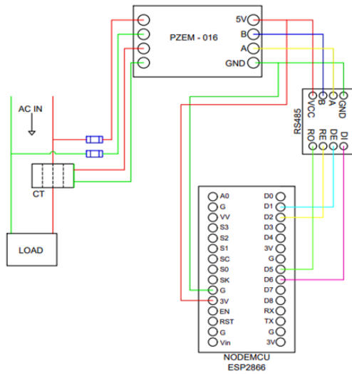
Fig.6. PZEM-016 to NodeMCU ESP8266 Wiring Diagram
