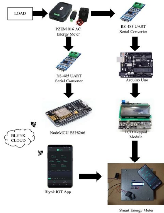
Fig. 5. Component Layout
