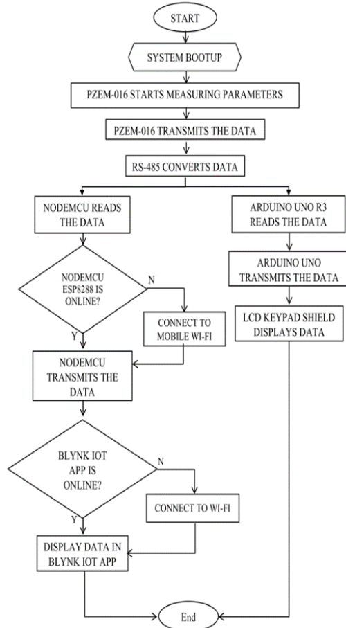
Fig.4. Program Flowchart
