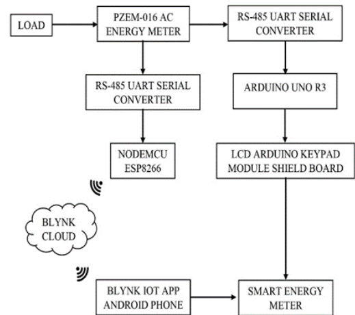
Fig. 3. Block Diagram
