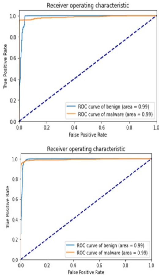
Fig.3. Receiver Operating Characteristic (Roc) Curves Of (Up) Malconv with Stretch Padding And (Down) Spapconv with Post Padding, Where Area Indicates Area Under the Curve (Auc) Score.
